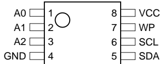
8-Pin TSSOP
